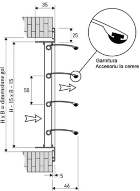
VK-B E Evacuare
