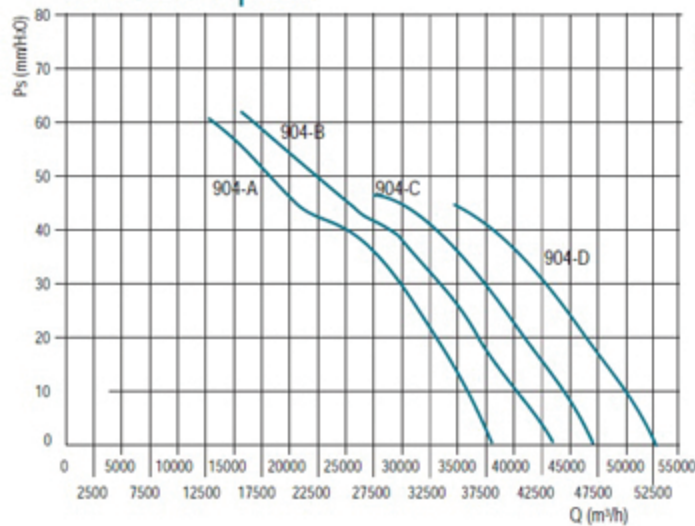
RING 1000 - 4 poles
