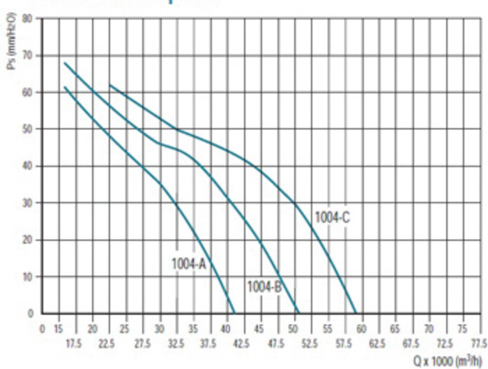
RING 1000 - 4 poles
